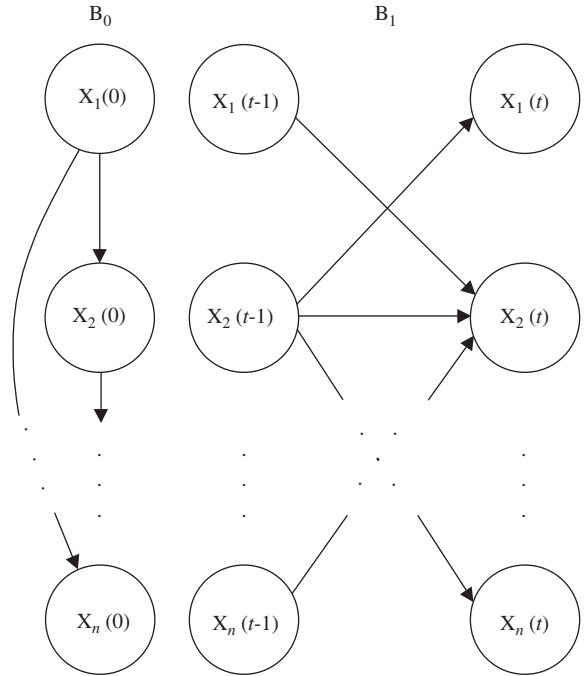
Fig. 2. An example of the basic building blocks of dynamic Bayesian networks (DBNs) (B_0, B_1) . B_0 and B_1 are the initial and transition Bayesian networks (BNs), respectively.
