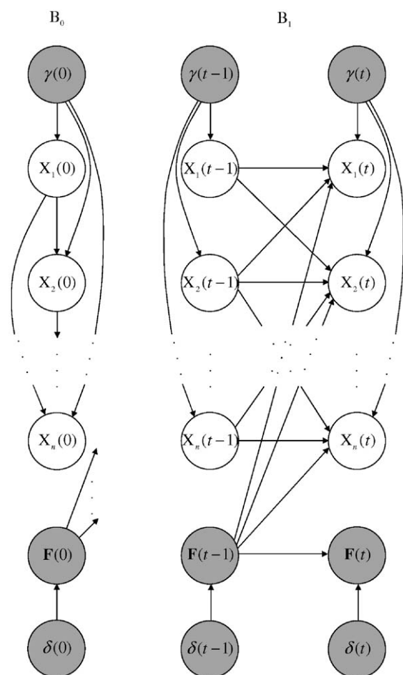
Fig. 5. Basic building blocks of a dynamic Bayesian network (DBN) allowing node perturbations and random network changes. B_0 and B_1 are the initial and transition Bayesian networks (BNs). The hidden variables \gamma(t) , \mathbf{F}(t) and \delta(t) are shown in gray.
