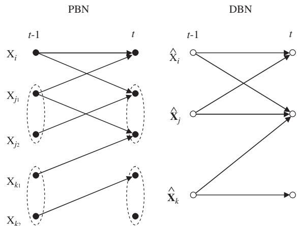
Fig. 3. Correspondence between the nodes in a dependent PBN and a DBN (see the text for details).
