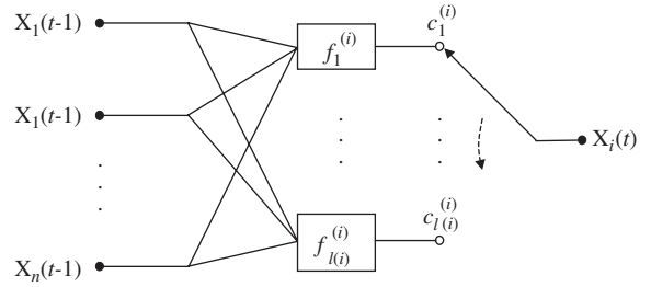
Fig. 1. A basic building block of probabilistic Boolean networks (PBN). The graph describes the updating mechanisms for a single node X_i in the network.
